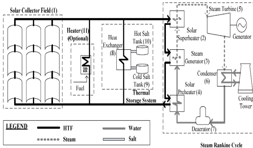
Figure 3 (Parabolic Trough Collector - PTC Configuration)
