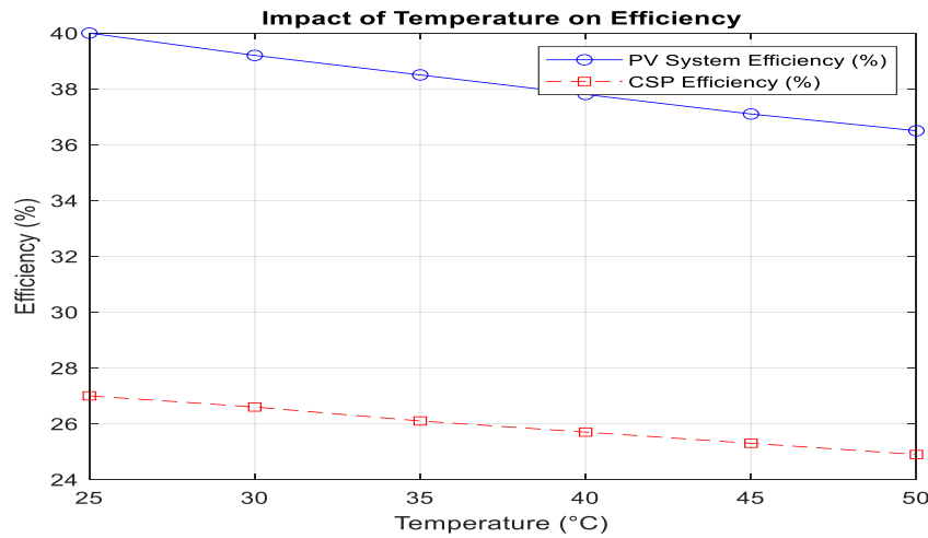
Figure 9 – Impact of Temperature on Efficiency
