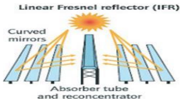
Figure 4 (Linear Fresnel Reflector - LFR Configuration)
